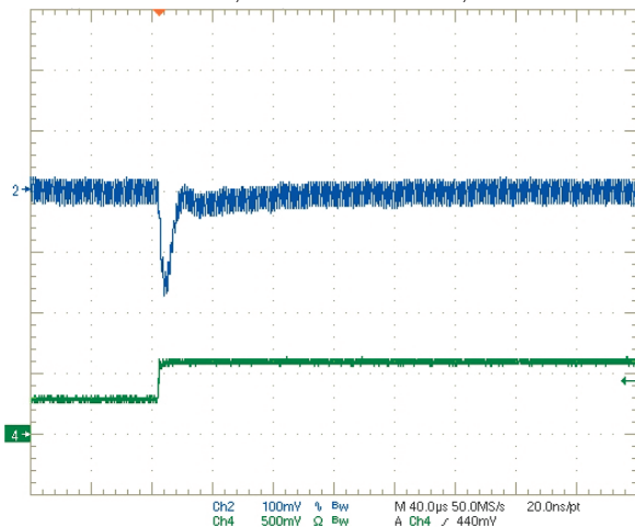
Step Load Transient Response (Vin=12V, Vout=2.5V, Clad=0, Iout=1.5A to 3A) Trace 2=Vout, 100 mV/div. Trace 4=Iout, 2.5A/div.
