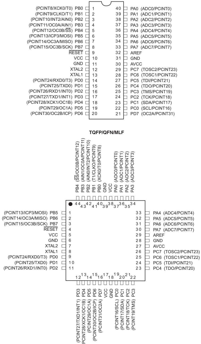
Figure 1-1. Pinout.
