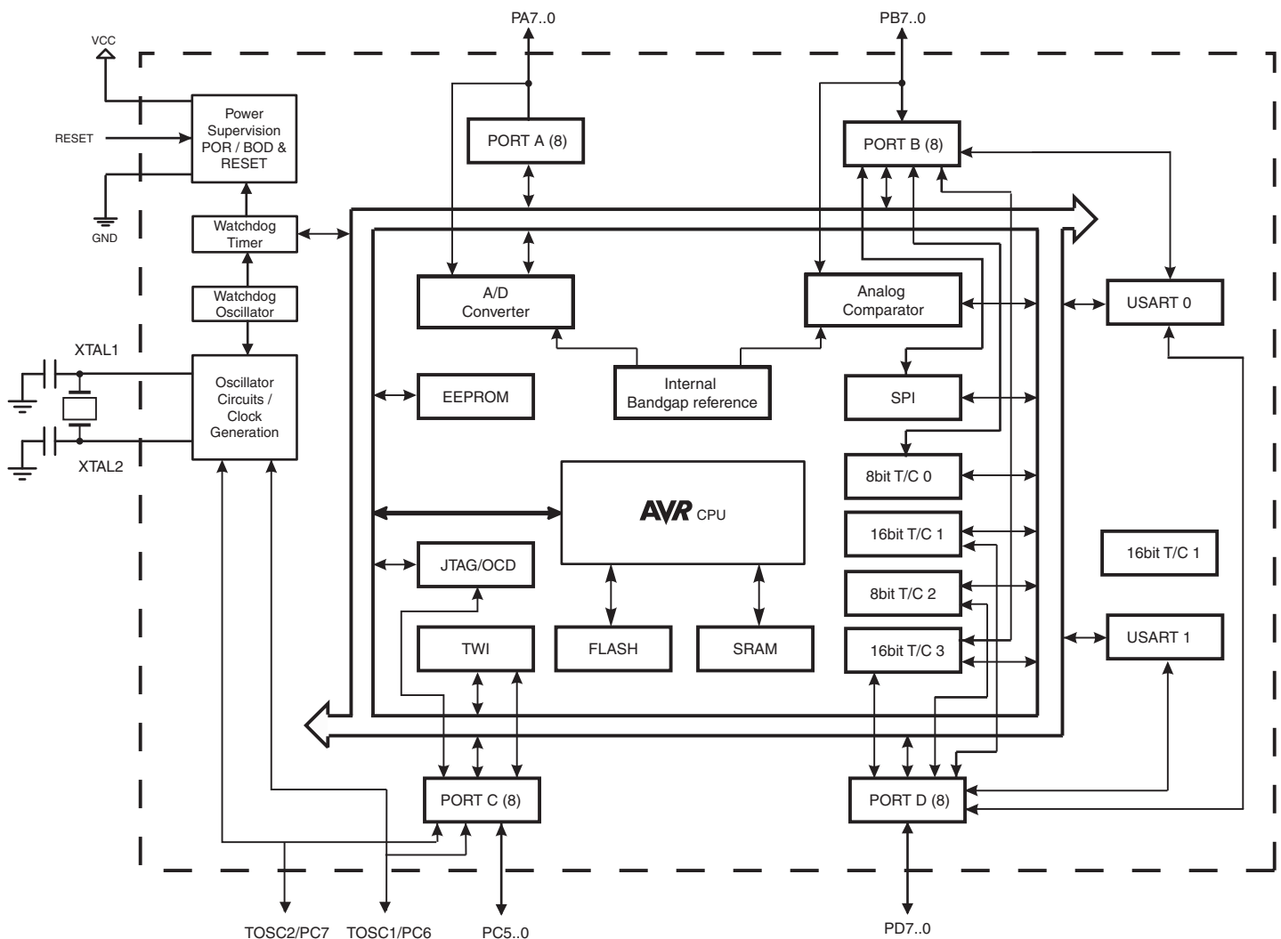
Figure 2-1. Block diagram.
