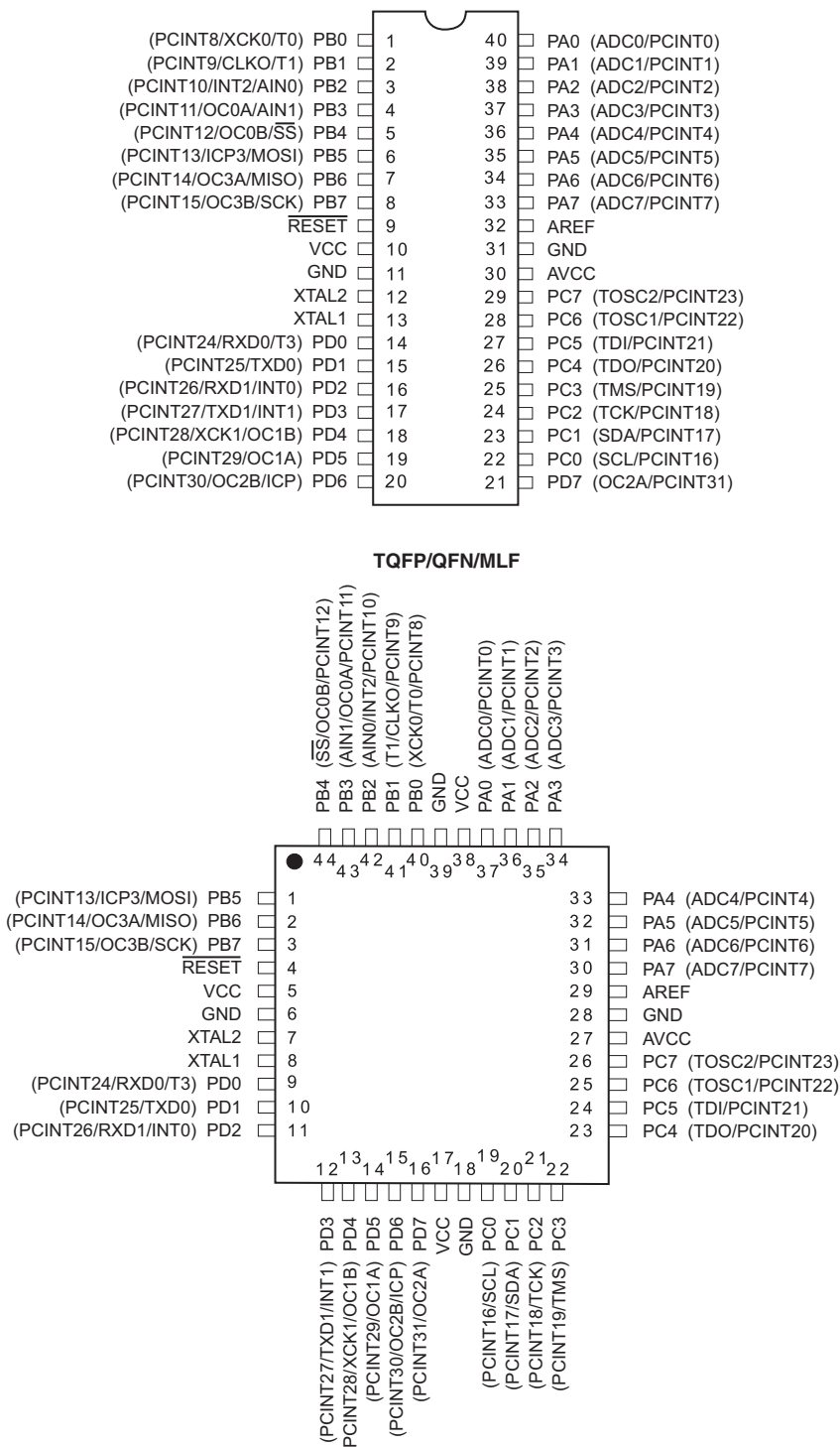
Figure 1-1. Pinout.
