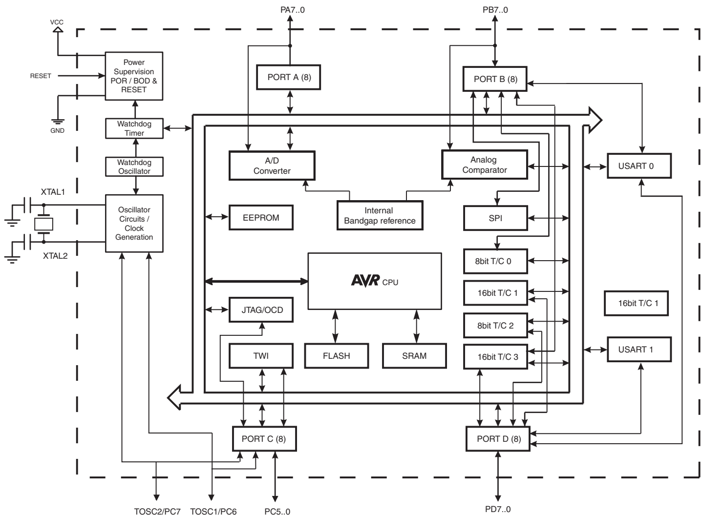
Figure 2-1. Block diagram.
