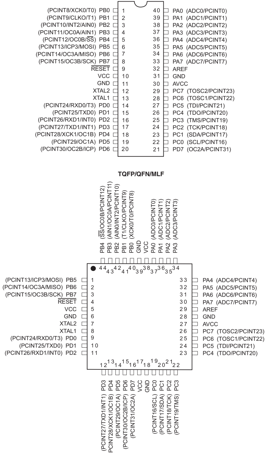
Figure 1-1. Pinout.
