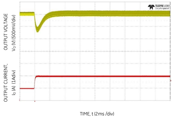
Figure 4. Transient Response to Dynamic Load Change from 50% to 100% at 12Vin, C_{out}=12 \times 4.7 \mu\text{F} , C_{Tune}=820\text{pF} , R_{Tune}=30.1\text{k}
