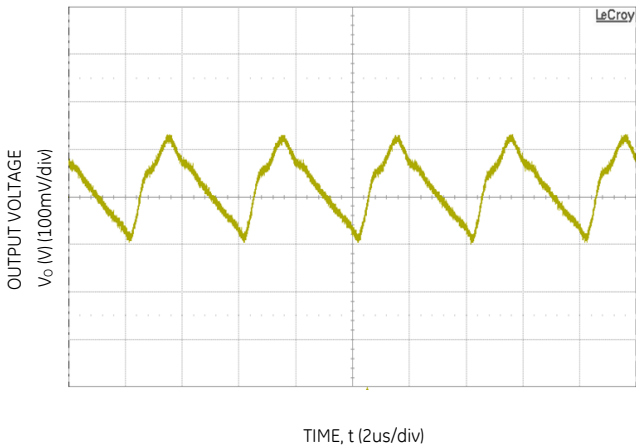
Figure 3. Typical output ripple and noise ( C_o=66 \mu\text{F} ceramic, V_{IN} = 12\text{V} , I_o = I_{o,max} ).
