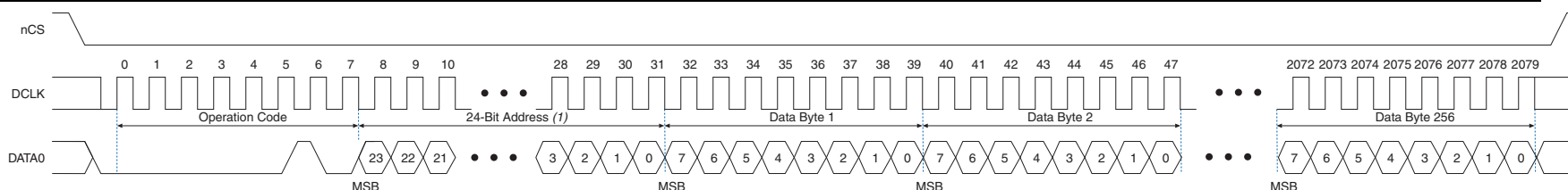
Figure 13. Write Bytes Operation Timing Diagram
