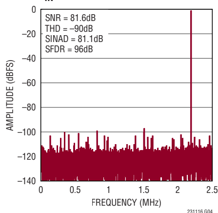
32k Point FFT, f_{SAMPL} = 5\text{Mps} , f_{IN} = 2.2\text{MHz}
