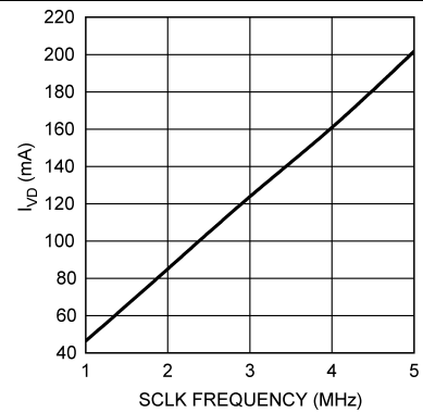
Figure 34. V_{IO} Current vs. SCLK Frequency
