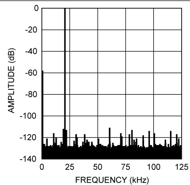
Figure 36. Spectral Response - 250 kSPS
