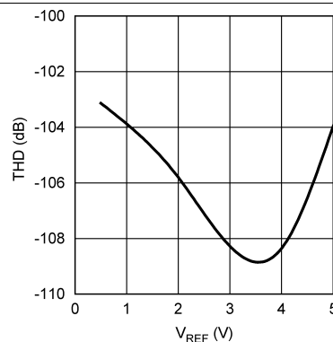
Figure 20. THD vs. V_{REF}
