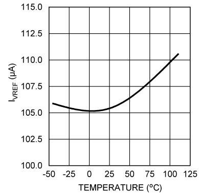
Figure 32. V_{REF} Current vs. Temperature
