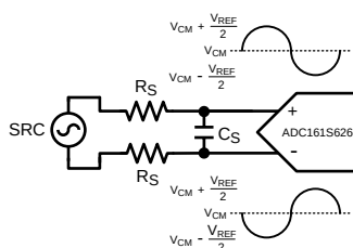
Figure 43. Differential Input
