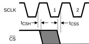
Figure 5. Valid \overline{\text{CS}} Assertion Times
