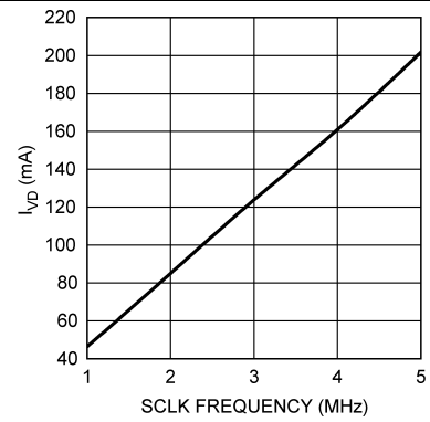
Figure 34. V_{IO} Current vs. SCLK Frequency
