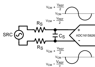
Figure 43. Differential Input
