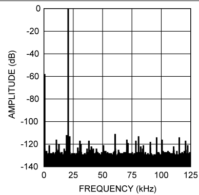
Figure 36. Spectral Response - 250 kSPS
