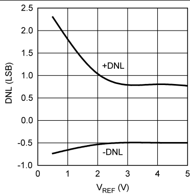
Figure 11. DNL vs. V_{REF}
