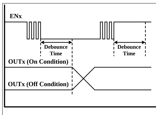
Figure 18 ENx Debounced
