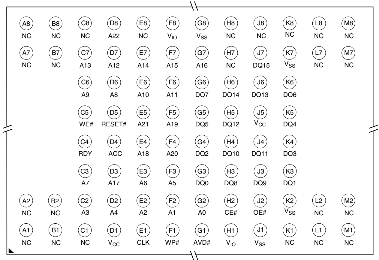
80-ball Fine-Pitch Ball Grid Array Top View, Balls Facing Down (Am29BDS128H only)
