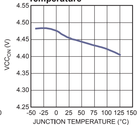
VCC Regulator On Threshold vs. Junction Temperature
