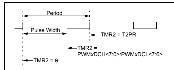
FIGURE 25-2: PWM OUTPUT
