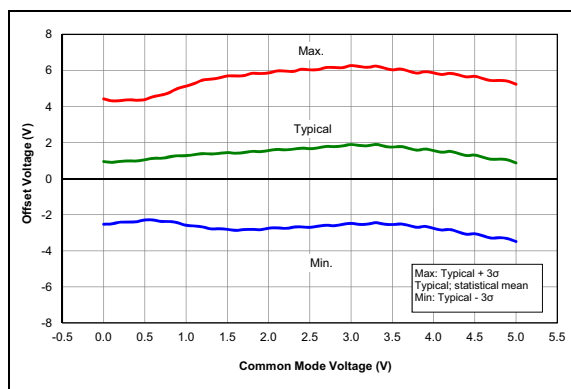
FIGURE 37-98: Op Amp, Offset over Common Mode Voltage, V_{DD} = 5.0V , Temp. = 25^\circ C , PIC16F1777/8/9 Only.
