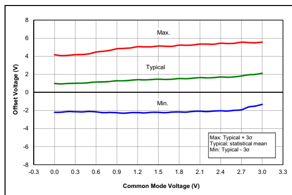
FIGURE 37-97: Op Amp, Offset over Common Mode Voltage, V_{DD} = 3.0V , Temp. = 25^\circ C
