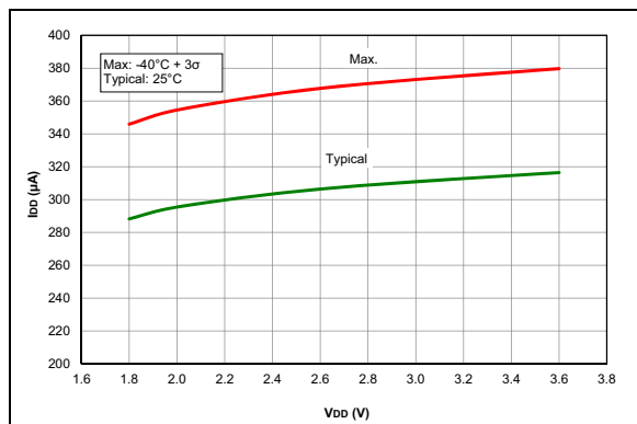
FIGURE 37-50: I_{D} , Comparator, NP Mode ( V_{REGPM} = 0 ), PIC16LF1777/8/9 Only.
