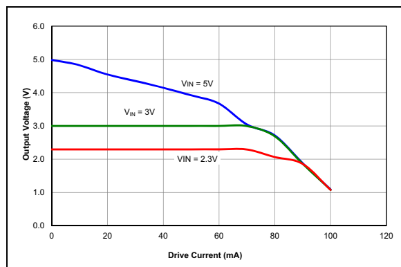
FIGURE 37-101: Op Amp, Output Drive Strength, V_{DD} = 5.0V , Temp. = 25^\circ C , PIC16F1777/8/9 Only.
