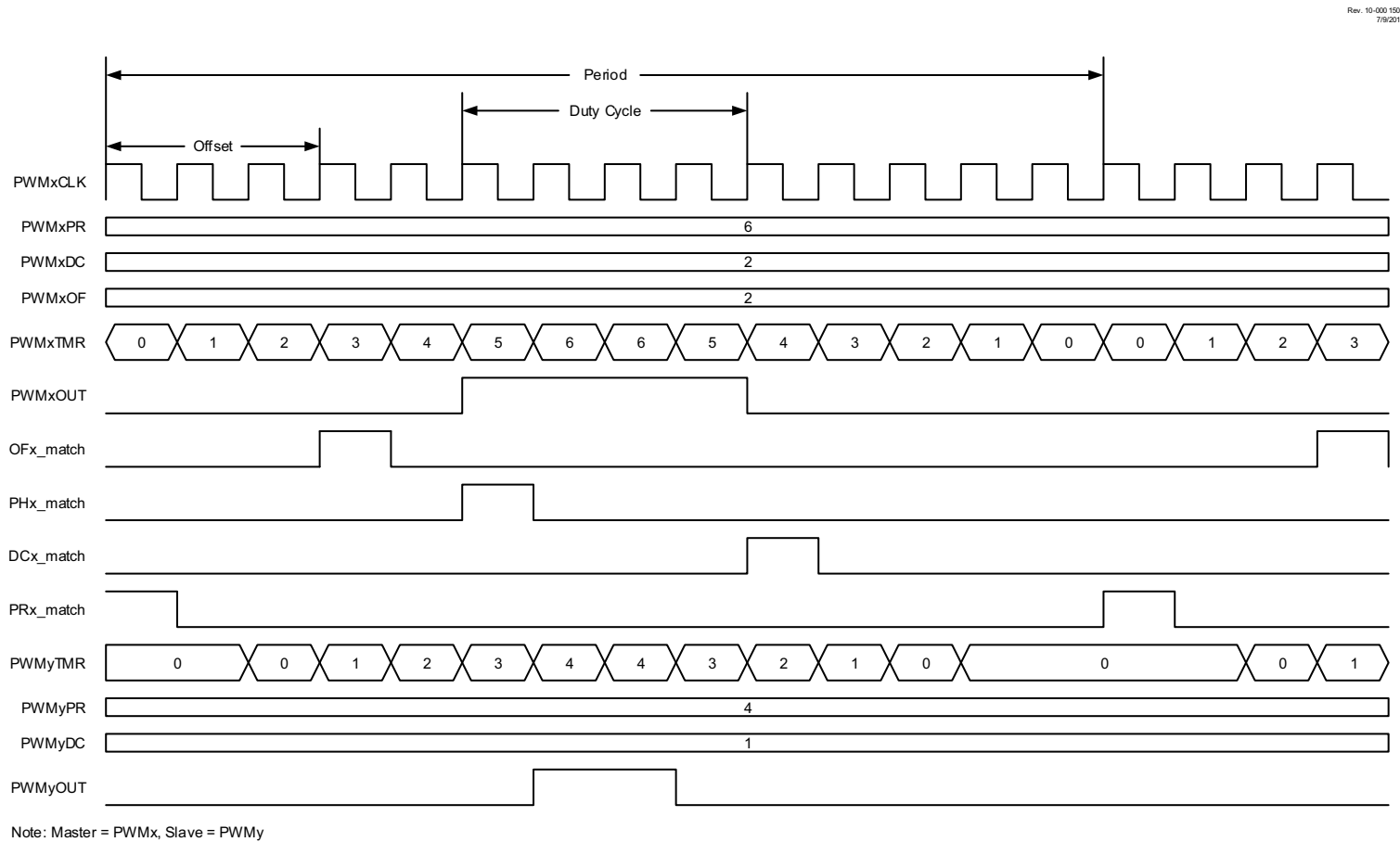
FIGURE 26-12: OFFSET MATCH ON INCREMENTING TIMER TIMING DIAGRAM
