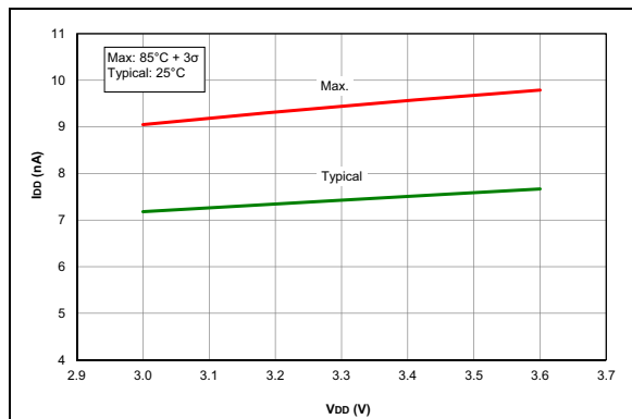
FIGURE 37-40: I_{DD} , Brown-Out Reset (BOR), BORV = 1, PIC16LF1777/8/9 Only.
