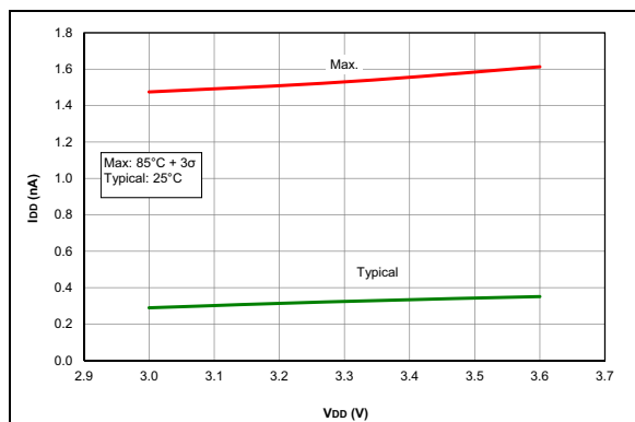
FIGURE 37-42: I_{DD} , LP Brown-Out Reset (LPBOR = 0), PIC16LF1777/8/9 Only.
