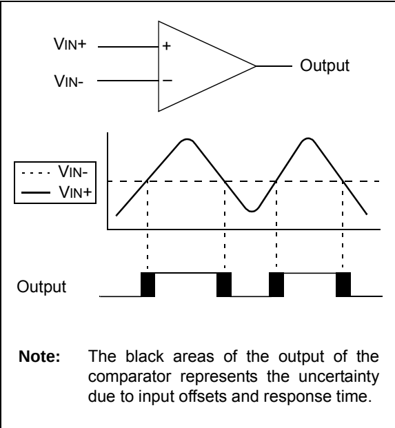
FIGURE 19-1: SINGLE COMPARATOR
