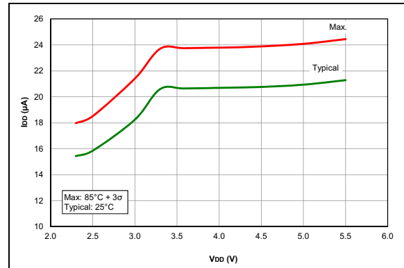
FIGURE 37-20: I_{DD} , LFINTOSC Mode, F_{osc} = 31\text{ kHz} , PIC16F1777/8/9 Only.
