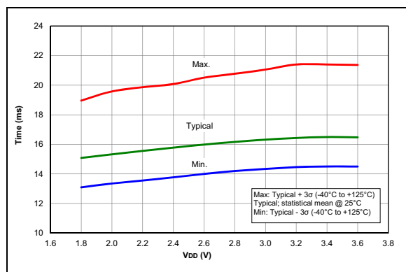
FIGURE 37-61: WDT Time-Out Period, PIC16LF1777/8/9 Only.
