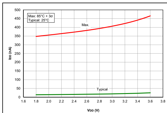
FIGURE 37-48: I_D , ADC Non-Converting, PIC16LF1777/8/9 Only.
