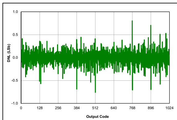
FIGURE 37-78: ADC 10-bit Mode, Single-Ended DNL, V_{DD} = 3.0V , T_{AD} = 1\text{ }\mu s , 25^\circ C .
