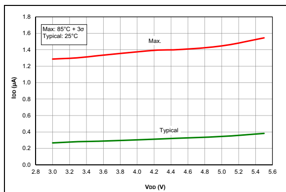
FIGURE 37-43: I_D , LP Brown-Out Reset ( LPBOR = 0 ), PIC16F1777/8/9 Only.
