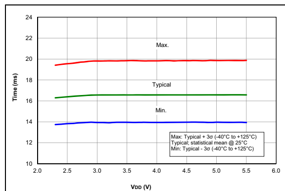
FIGURE 37-60: WDT Time-Out Period, PIC16F1777/8/9 Only.
