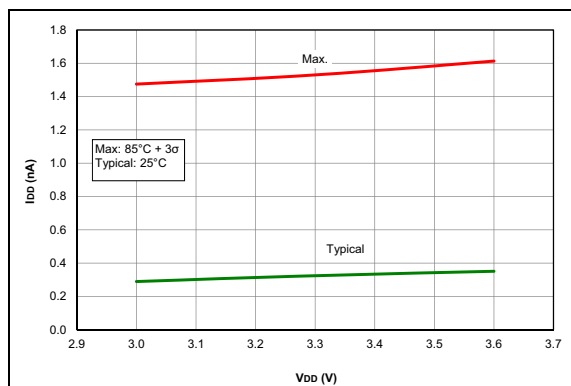
FIGURE 37-42: I_{PD} , LP Brown-Out Reset (LPBOR = 0), PIC16LF1777/8/9 Only.
