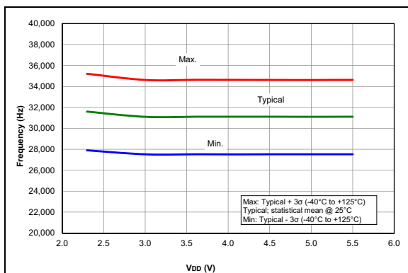
FIGURE 37-59: LFINTOSC Frequency, PIC16F1777/8/9 Only.
