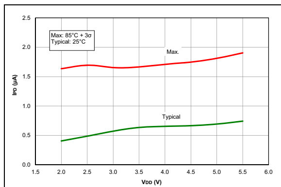
FIGURE 37-35: I_{PD} , Watchdog Timer (WDT), PIC16F1777/8/9 Only.
