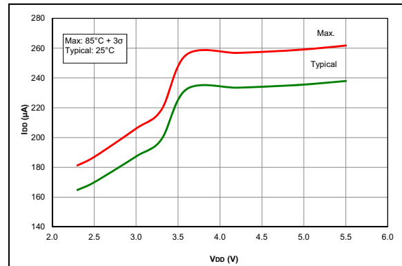
FIGURE 37-22: I_{DD} , MFINTOSC Mode, F_{osc} = 500\text{ kHz} , PIC16F1777/8/9 Only.
