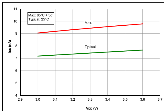
FIGURE 37-40: I_{PD} , Brown-Out Reset (BOR), BORV = 1, PIC16LF1777/8/9 Only.
