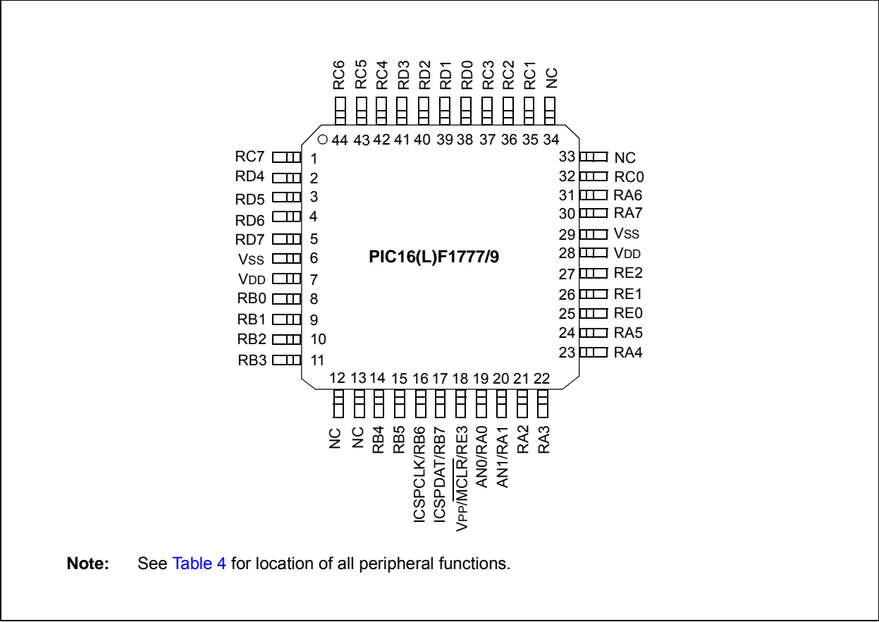
FIGURE 6: 44-PIN QFN (8X8 mm)
