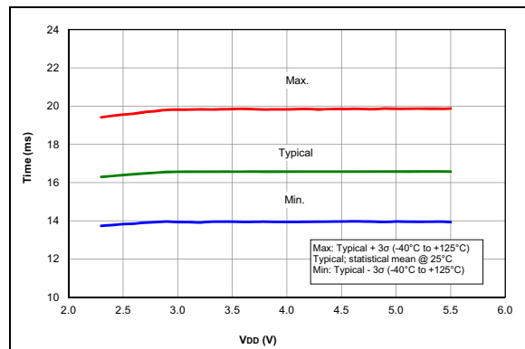
FIGURE 37-60: WDT Time-Out Period, PIC16F1777/8/9 Only.
