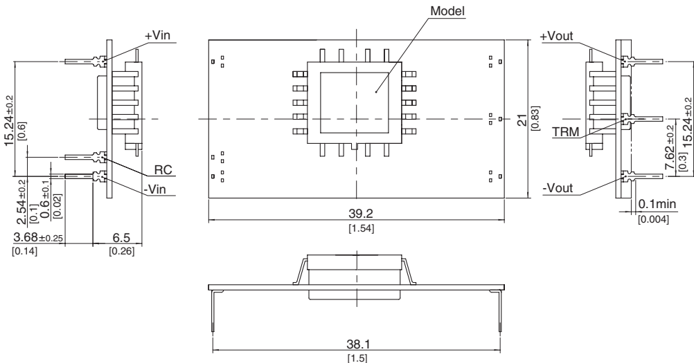
2. DIP(type C)
