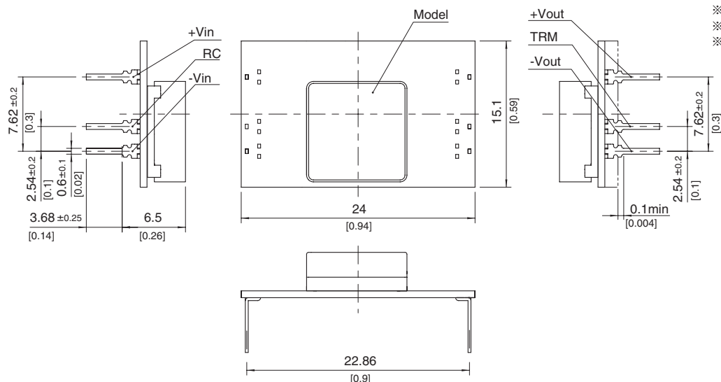
2.DIP(type C)
