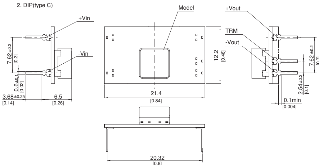
2. DIP(type C)
