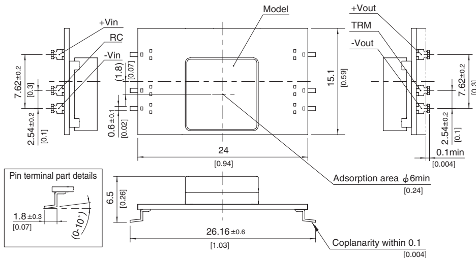
1. SMD(type B)
