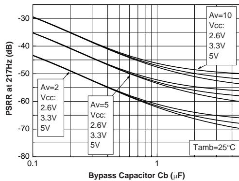
Figure 24. PSRR at F = 217 Hz vs. bypass capacitor
