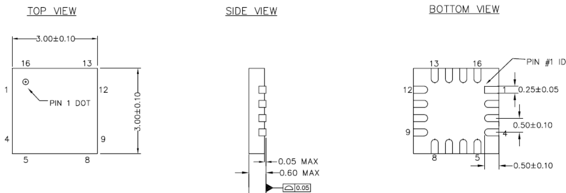
Figure 17. 16-pin QFN No Center Pad (3 x 3 x 0.6 mm) Package Outline (Sawn)
