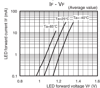
LED forward current vs. LED forward voltage
