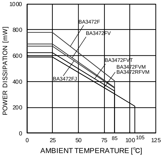
Figure 2. Derating Curve
