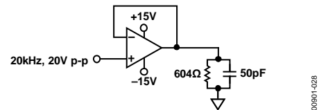
Figure 28. Output Swing, V_S = \pm 15\text{ V} , G = +1
