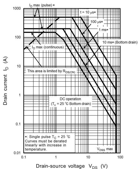
Fig. 8.16 Safe Operating Area (Guaranteed Maximum)
