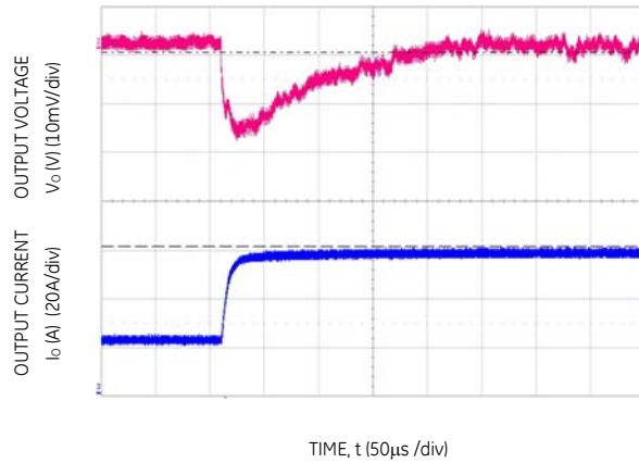
Figure 10. Transient Response to Dynamic Load Change from 25% to 75% at 12Vin, C_o = 30 \times 47\mu F + 11 \times 1000\mu F , R_{TUNE} = 3.74k\Omega
