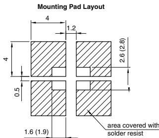
Dimensions: IR and Vaporphase (Wave Soldering)
