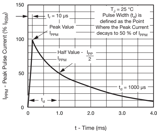
Fig. 3 - Pulse Waveform
