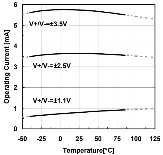
Operating Current vs. Temperature V_{IN}=0V, no\ load
