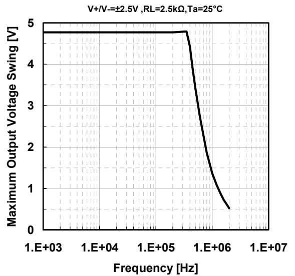
Maximum Output Voltage Swing vs. Frequency V+/V- = \pm 2.5V , R_L = 2.5k\Omega , T_a = 25^\circ C
