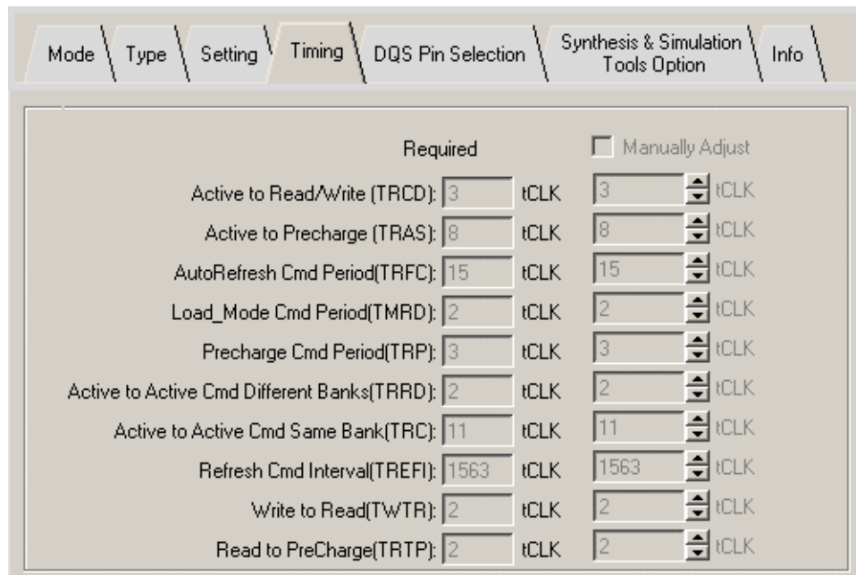
Figure 3-5. Timing Tab
