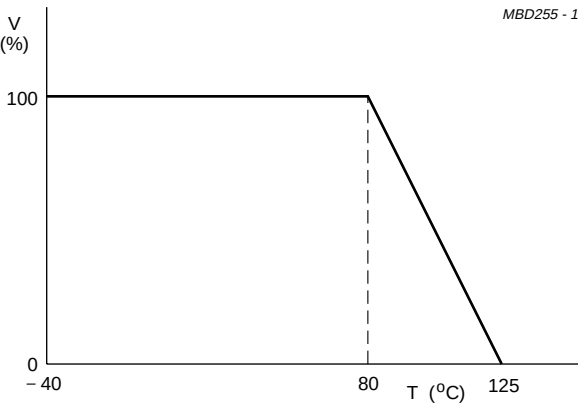
Fig.12 Derating curve.
