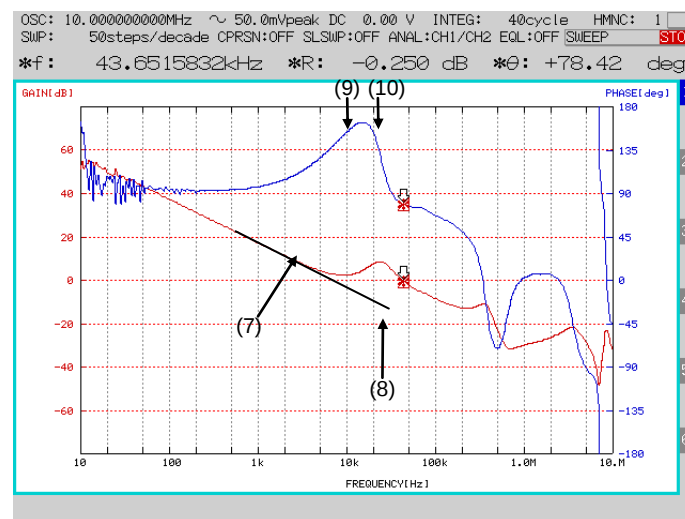
Figure 37. Example of DC/DC Converter Frequency Property (Measured with FRA5097 by NF Corporation)
