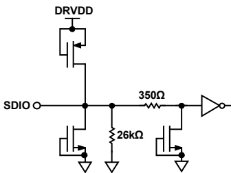
Figure 42. Equivalent SDIO Circuit
