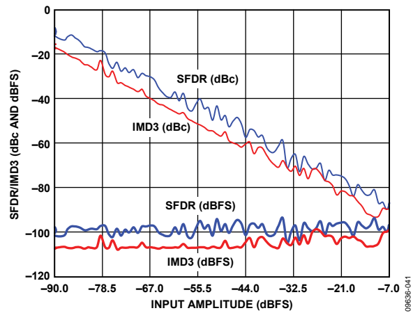
Figure 34. AD9643-250 Two-Tone SFDR/IMD3 vs. Input Amplitude ( A_{IN} ) with f_{IN1} = 184.12 , f_{IN2} = 187.12 MHz, f_s = 250 MSPS
