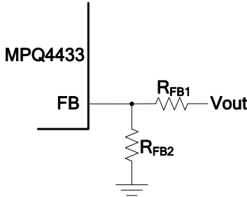
Figure 5: Feedback Network
