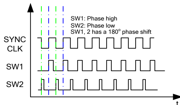
Figure 4: In-Phase and 180° Out-of-Phase
