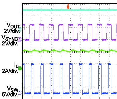
SYNC Operation (In-Phase)
