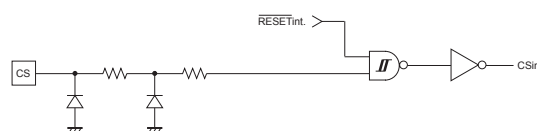
Input circuit
