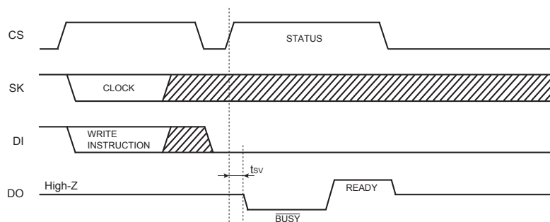
Fig. 54 R/\overline{B} status output timing chart
