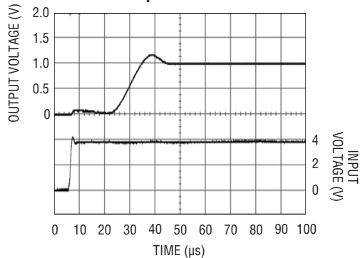
Turn-On Response
