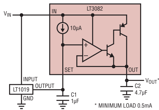
Reference Buffer
