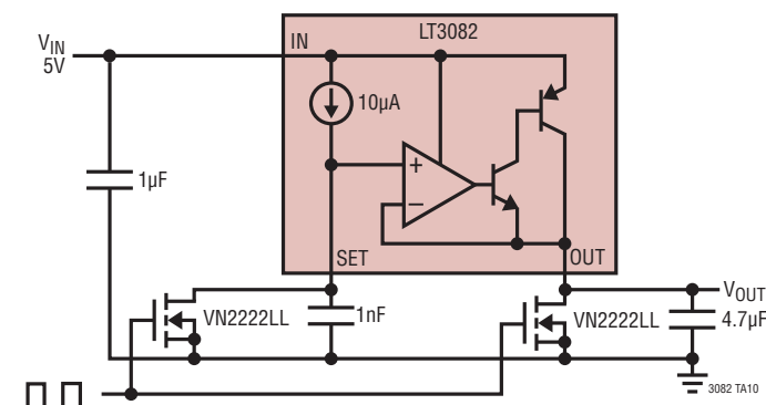
Ramp Generator
