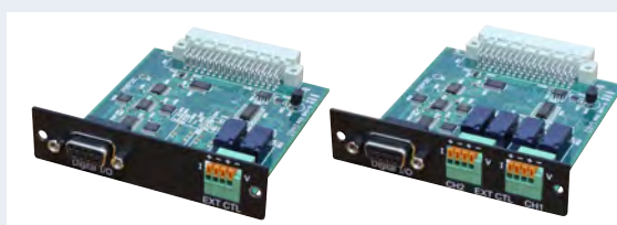
Single and dual channel digital I/O analog input control cards
