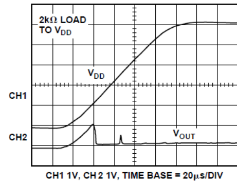
Figure 20. Power-On Reset to 0 V
