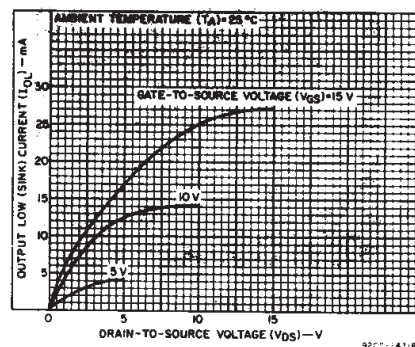
Fig. 3 - Typical n-channel output low (sink) current characteristics.
