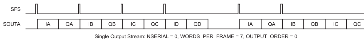
Figure 1-15. Serial Output Formats
