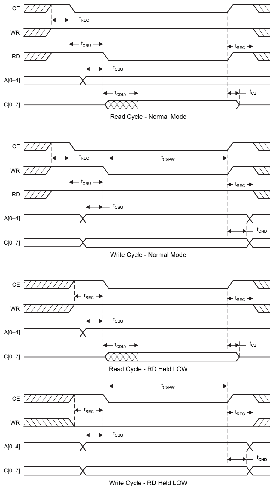
Figure 1-2. Normal Control I/O Timing
