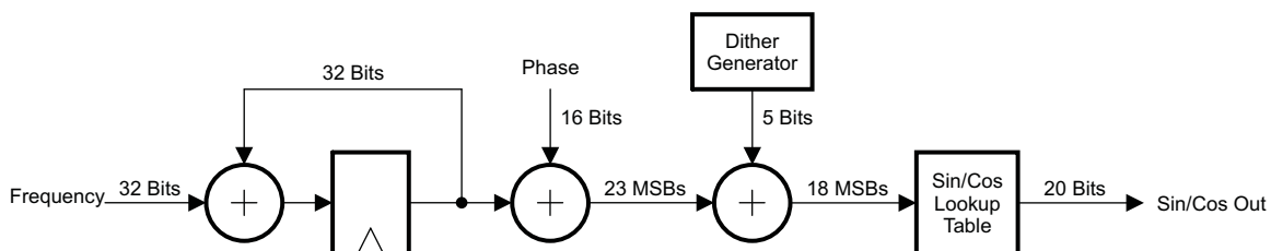
Figure 1-6. NCO Circuit
