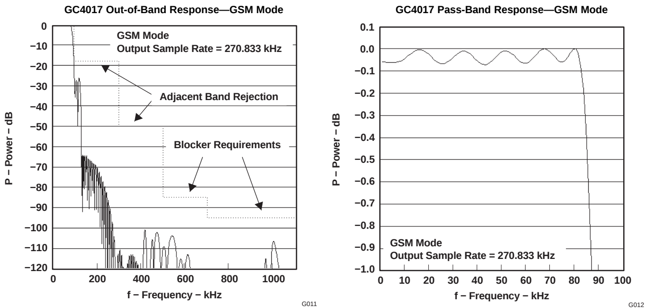
Figure 5-7. Frequency Response for the Example GSM Application
